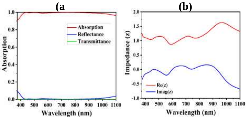
Figure 2. (a) Absorption spectra of PMA, (b) Effective impedance (Real and Imaginary) of the proposed absorber
