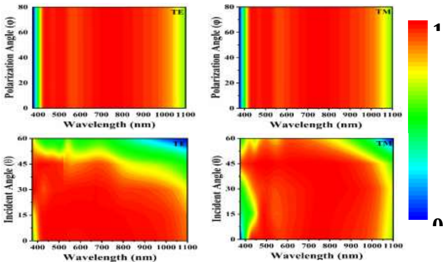
Figure 6. (a)-(b) Normal and oblique polarization angle from 0^{\circ} - 80^{\circ} , and (c)-(d) Normal and oblique incident angle from 0^{\circ} - 60^{\circ} for TE and TM modes, respectively.
