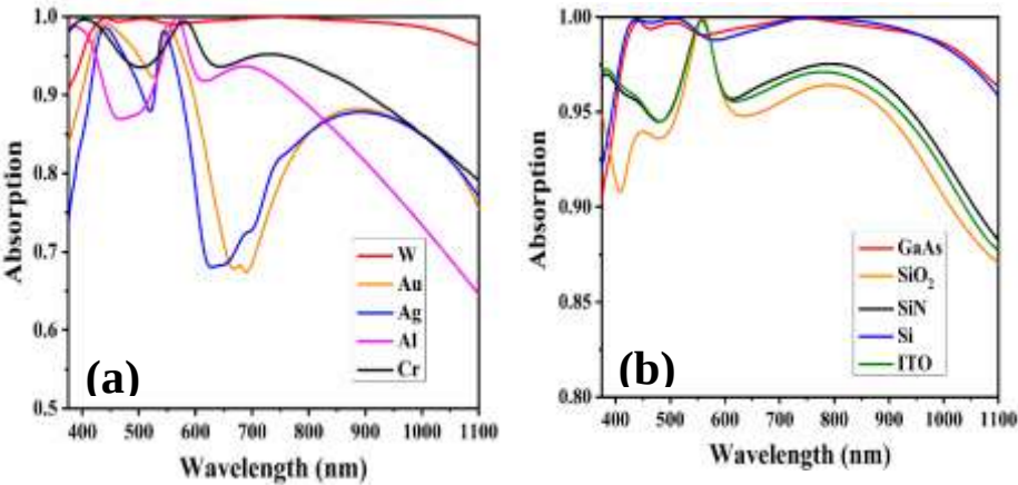
Figure 7. Absorption spectra of the absorber, (a) different metals of the bottom layer, and (b) different dielectric layers.
