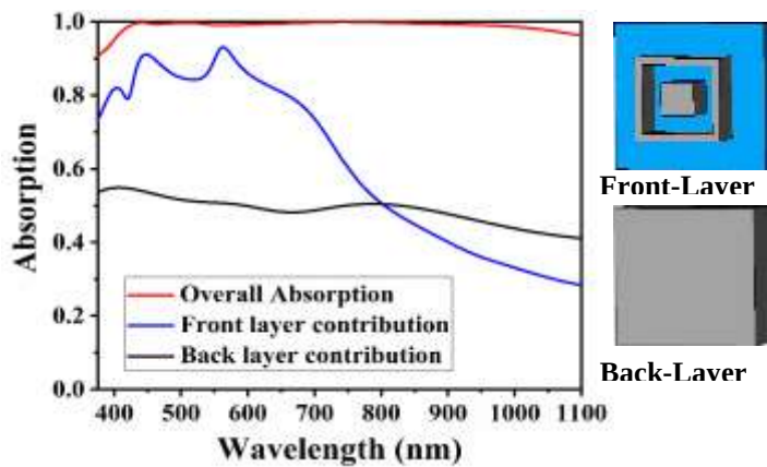
Figure 3. Absorption spectra withback-layer of tungsten metal, and front-layer (dielectric and resonator).
