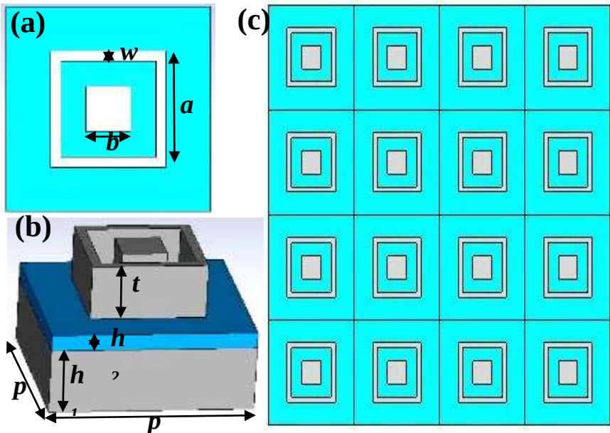
Figure 1. (a) A front view of the absorber, (b) A schematic design of the proposed absorber, (c) Unit cells structure in periodic range.
