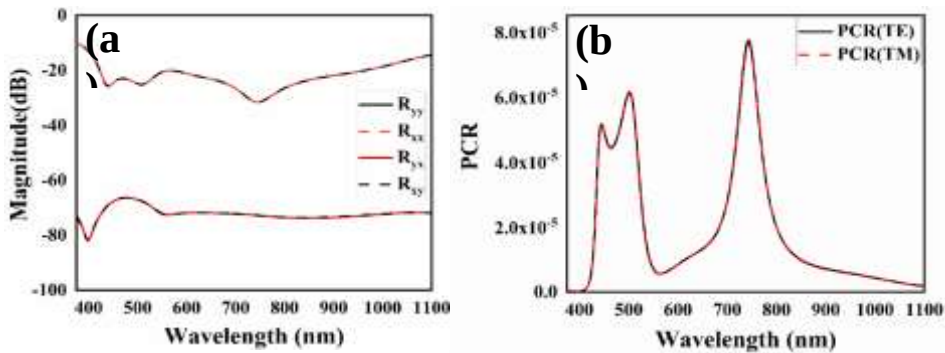
Figure 4. (a) Cross-polarization and Co-polarization components in magnitude (dB), (b) PCR for TE and TM mode.
