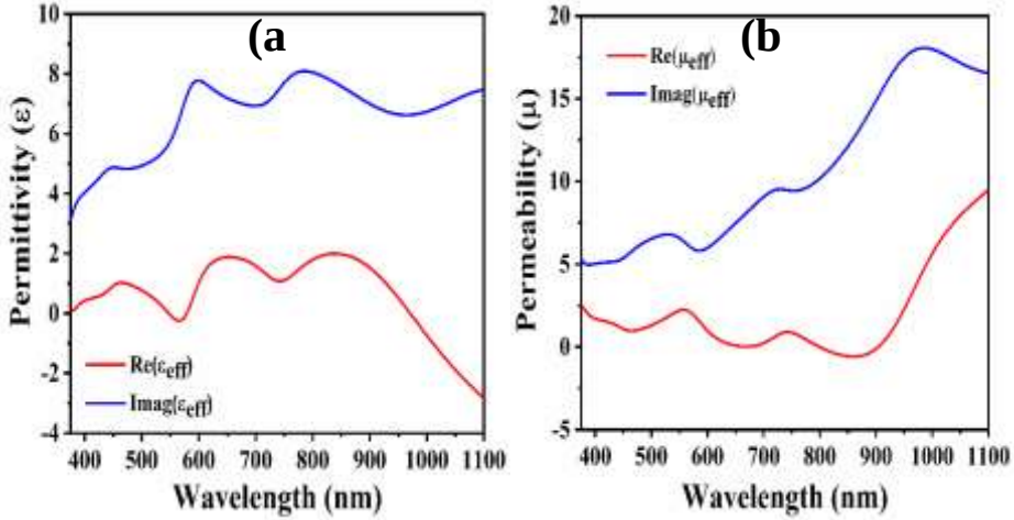
Figure 8. Extracted constitutive electromagnetic parameters of the absorber, (a) real and imaginary permittivity, and (b) real and imaginary permeability
