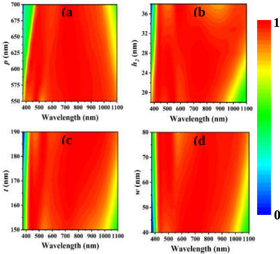
Figure 5. Absorption performances with structural parameters. (a) Period ( P ), (b) Thickness ( h_2 ) of the dielectric, (c) Thickness ( t ) of the resonator, and (d) Width ( w ) of the ring-shaped resonator.
