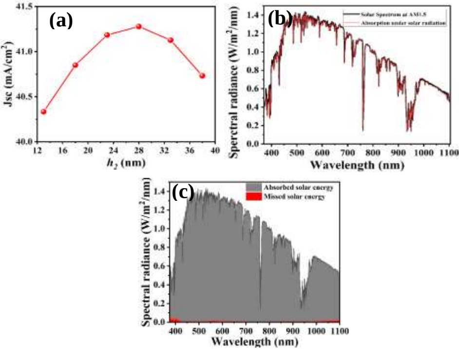
Figure 10. (a) Calculated short circuit current density ( J_{sc} ) with different thickness ( h_2 ) of GaAs layer, (b) Absorbed energy of proposed absorber in AM1.5 solar spectrum, (c) Absorbed solar energy and missed solar energy in the applied range of solar radiance.
