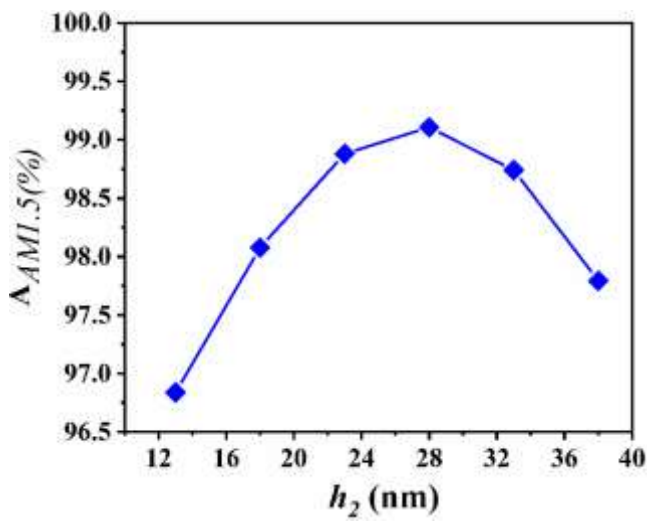
Figure 9. The conversion efficiency ( A_{AM1.5} ) with the various thickness ( h_2 ) of the dielectric layer
